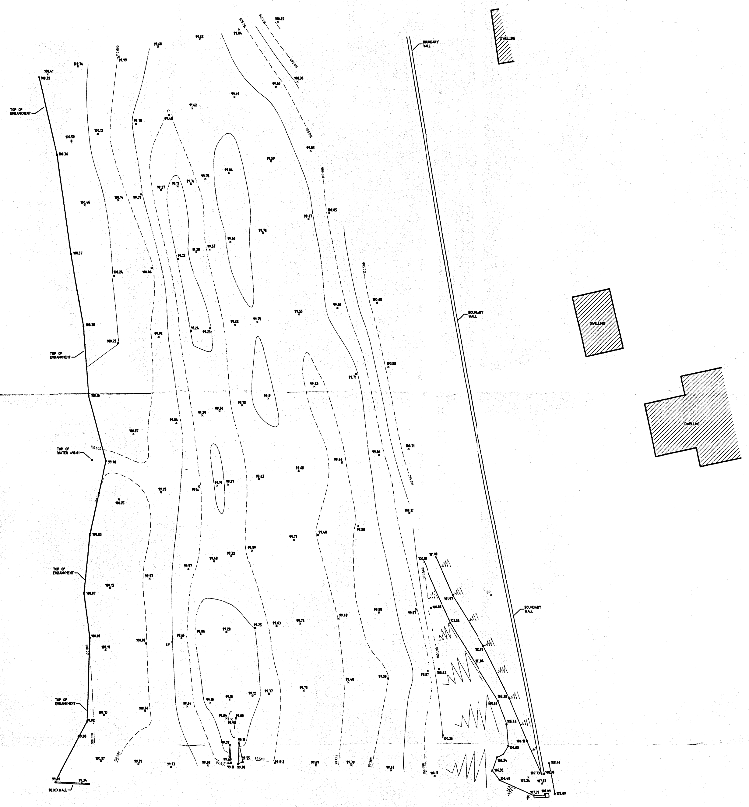
EXISTING SITE LAYOUT - SCALE 1:500
